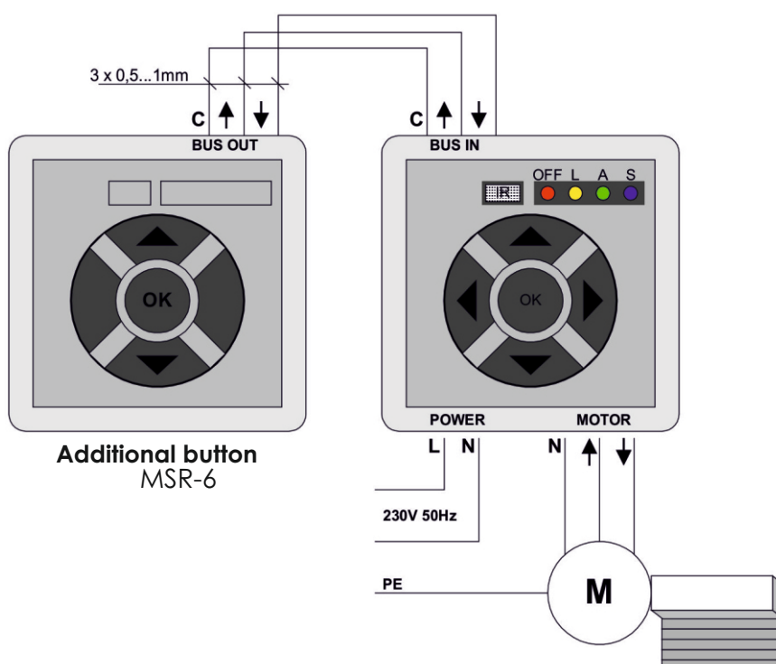
Diagram no. 2 MSR-3 version with additional button MSR-6
