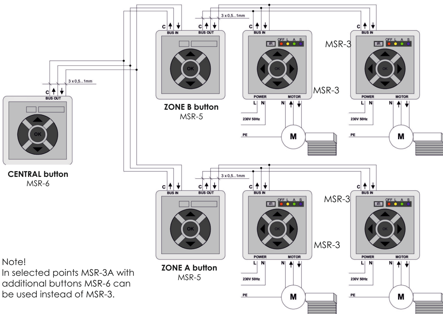
Diagram no. 4 System with division into two zones A and B (2 x MSR-5 + 2 x (n x MSR-3)) version with additional central button MSR-6
